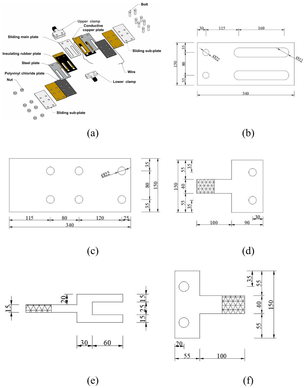
Figure S1. Specific design dimensions of the self-sensing damper. (a) Structural disassembly exploded view; (b) Sliding main plate, positive triboelectric plate, insulating layer, positive conductive layer; (c) Sliding sub-plate, negative triboelectric plate, negative grounding layer; (d) Sliding main plate's clamp (front view); (e) Sliding main plate's clamp (vertical view); (f) Sliding sub-plate's clamp.
