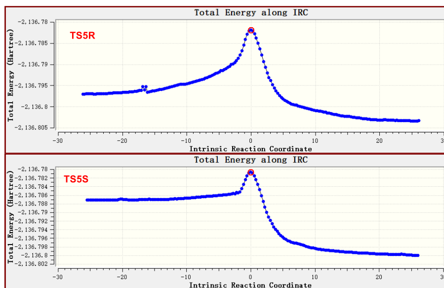
Figure S1. IRC calculations for the key stereoselective transition states TS5R and TS5S
