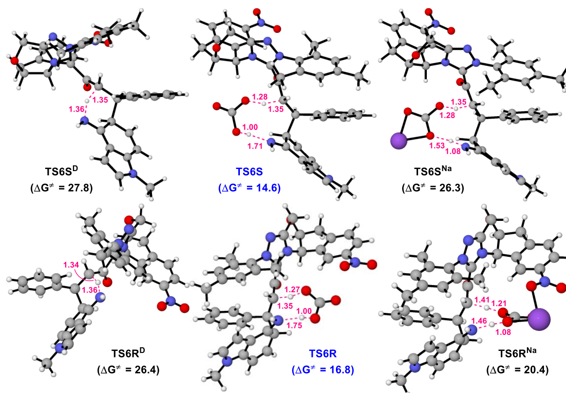
Figure S4. 3D structures and energy barriers for the transition states involving \alpha -protonation process
