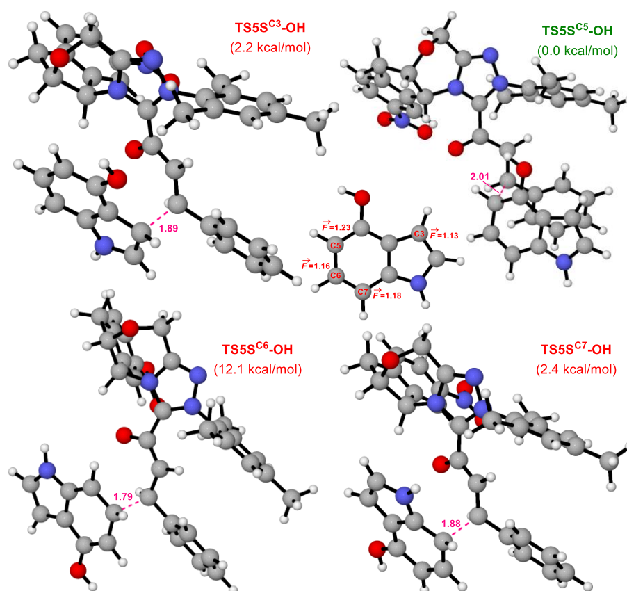
Figure S6. POCV results of intermediate M4 and 4-hydroxyindole
