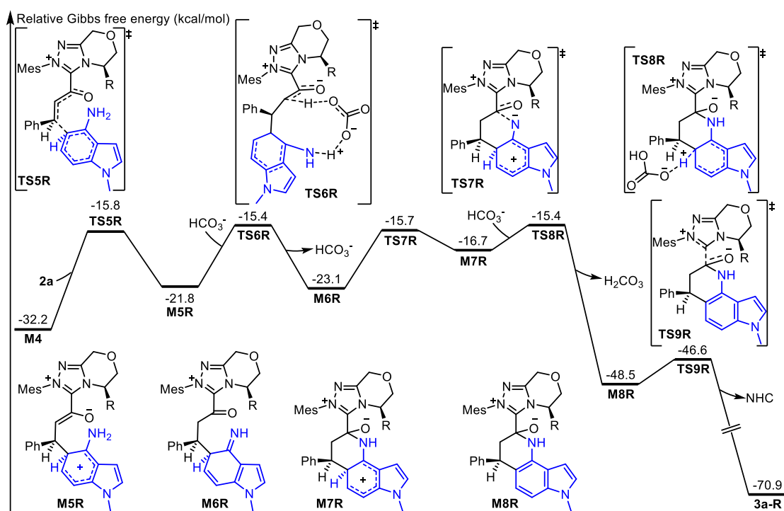
Figure S2. Relative Gibbs free energy profile for the transformation of \alpha,\beta -unsaturated acylazolium intermediate involved in R -configured pathway
