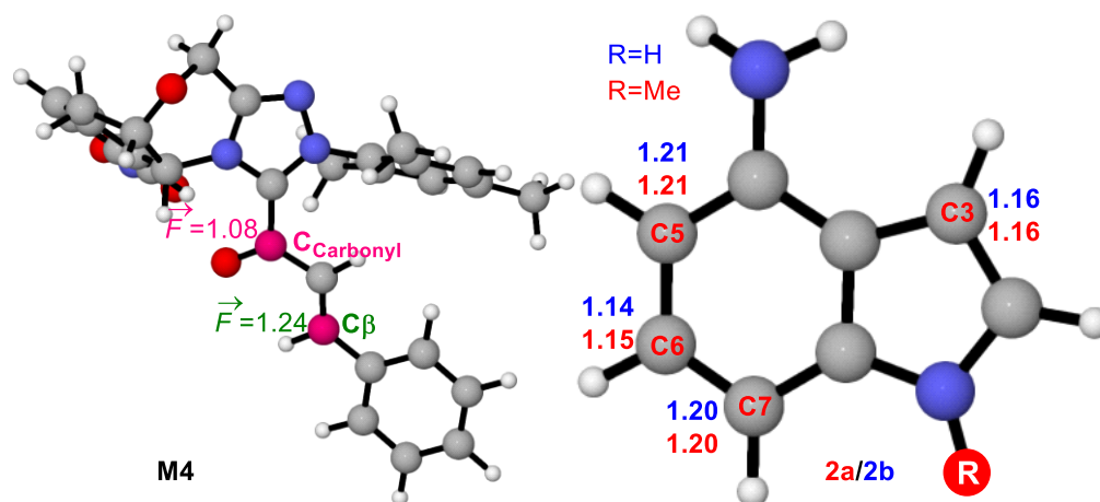
Figure S5. POCV results of intermediate M4 and 4-aminoindole
