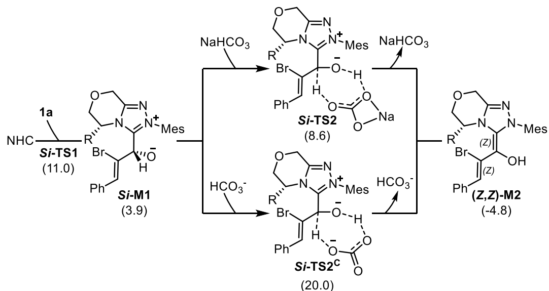
Scheme S1. \text{HCO}_3^- and \text{NaHCO}_3 -assisted proton transfer pathways
