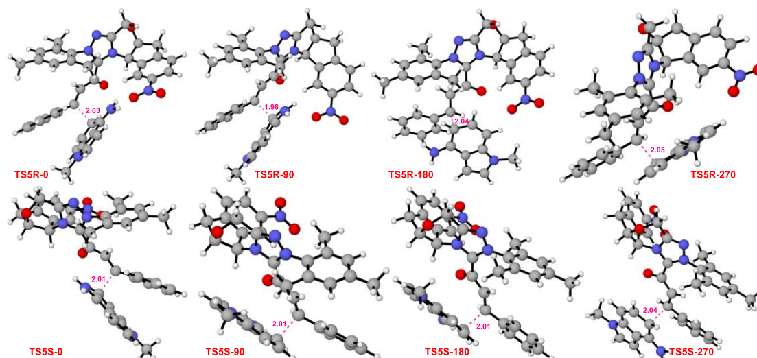
Figure S3. 3D structures for transition states TS5R and TS5S
