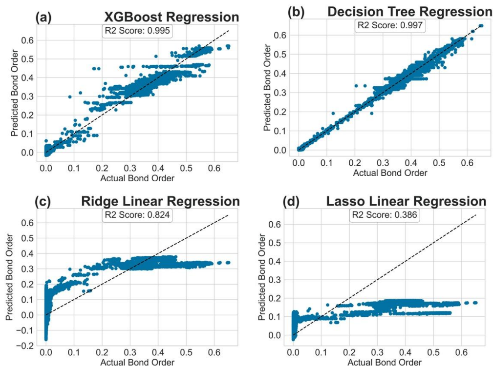
Figure S1. R2 plot for regression models tested. (a) XGBoost regression; (b) Decision tree regression; (c) Ridge linear regression; (d) Lasso linear regression in Setting (C).
