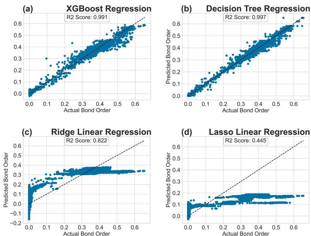
Figure S2. R2 plot for regression models tested. (a) XGBoost regression; (b) Decision tree regression; (c) Ridge linear regression; (d) Lasso linear regression in Setting (D).
